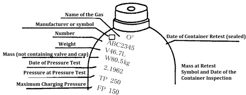
Figure 34. Cylinder Display
